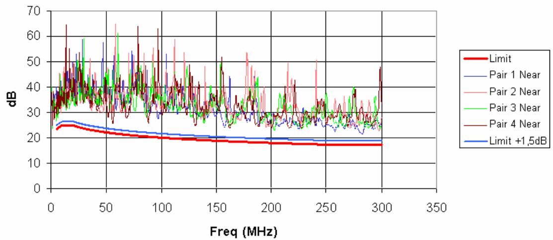
SAMPLE Return Loss Near End
