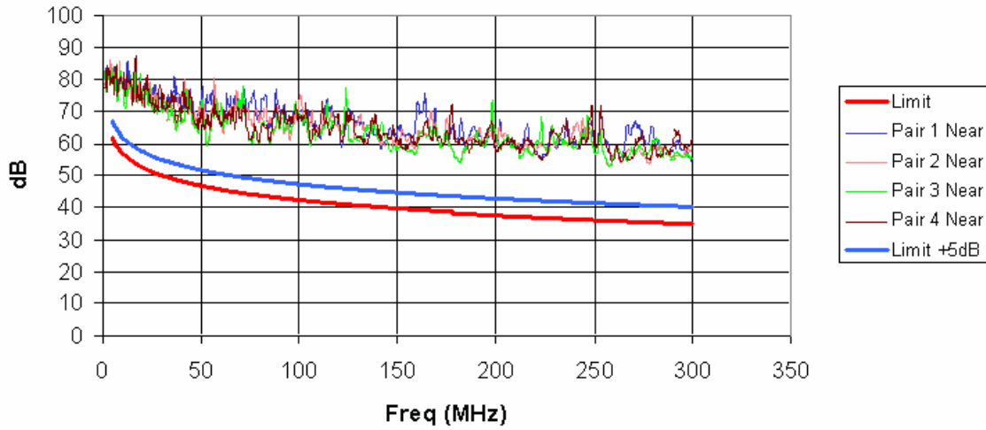
SAMPLE PS NEXT Near End
