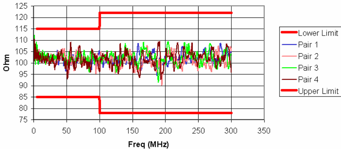
SAMPLE Characteristic Impedance Near End
